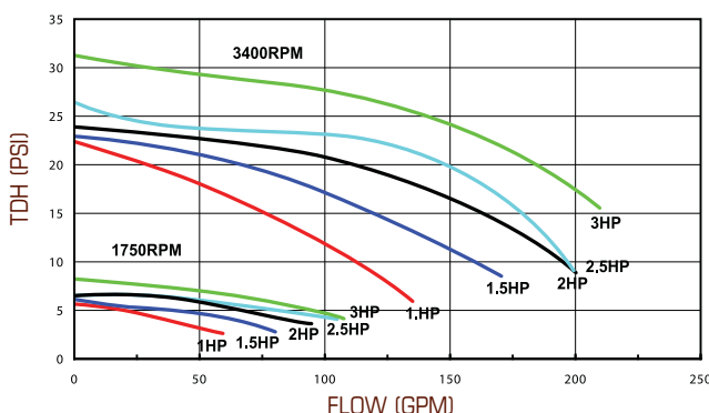
60Hz PERFORMANCE CURVE North America Model
