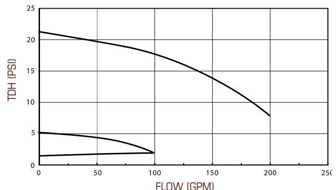
50Hz PERFORMANCE CURVE International Model
