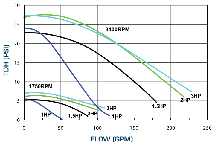
60Hz PERFORMANCE CURVE USA Model
